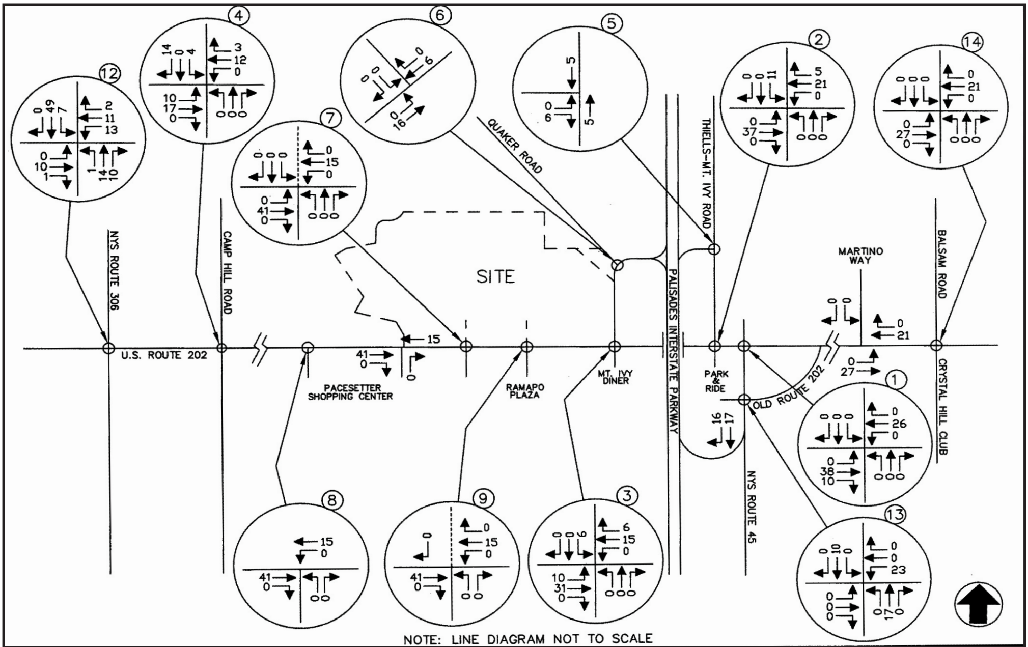
Figure 3.5-9: Other Development Traffic Volumes Weekday Peak PM Highway Hour (W/O Patrick Farm) Minisceongo Park Towns of Haverstraw & Ramapo, Rockland County, New York Source: John Collins Engineers, P.C. Date: October, 2008
